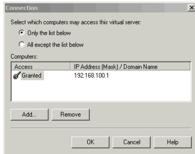
Figure 35 Connection Dialog Box for SMTP
