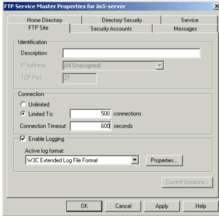
Figure 11 FTP Site Master Properties Sheet
